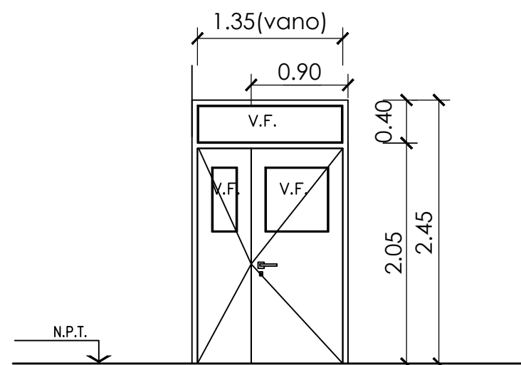
VISTA FRONTAL
