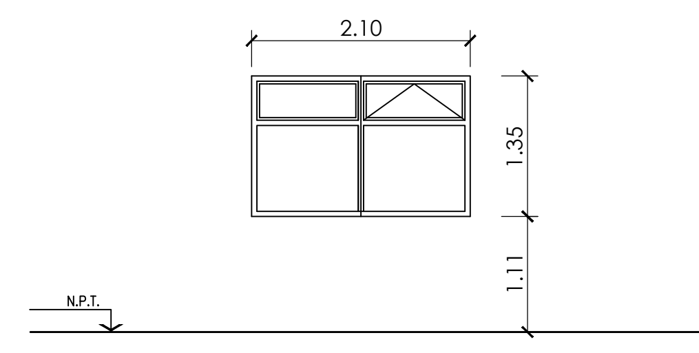
VISTA FRONTAL
