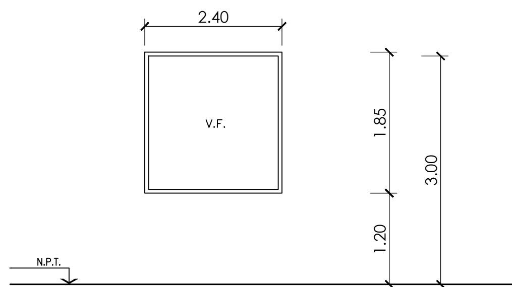
VISTA FRONTAL
