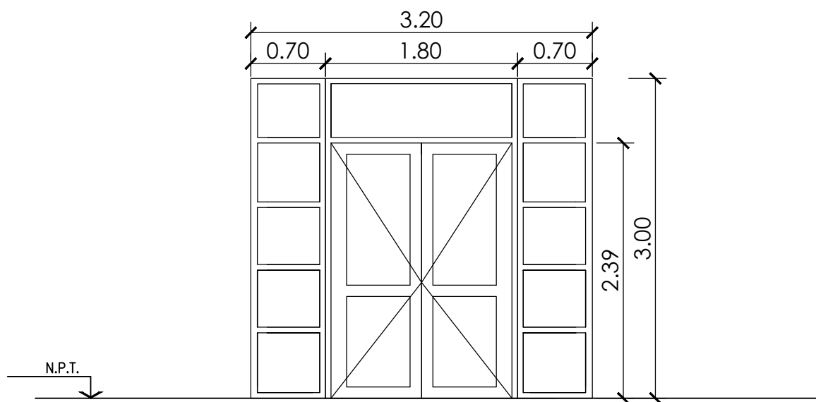
VISTA FRONTAL
